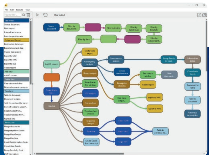
Workflow Editor
