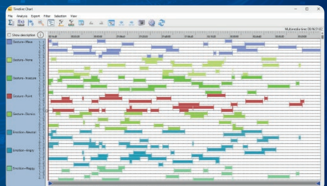
Timeline Chart
